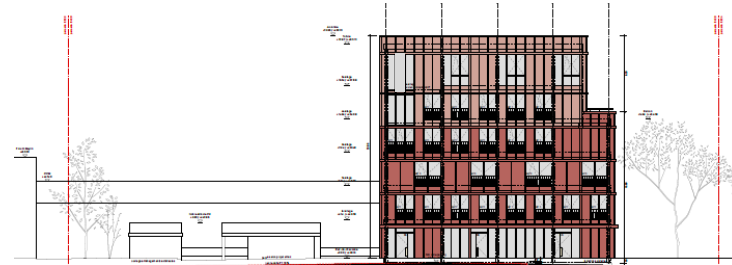
FACADE TRAM
